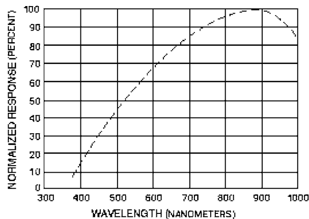
Typical response of Detector versus wavelength.
