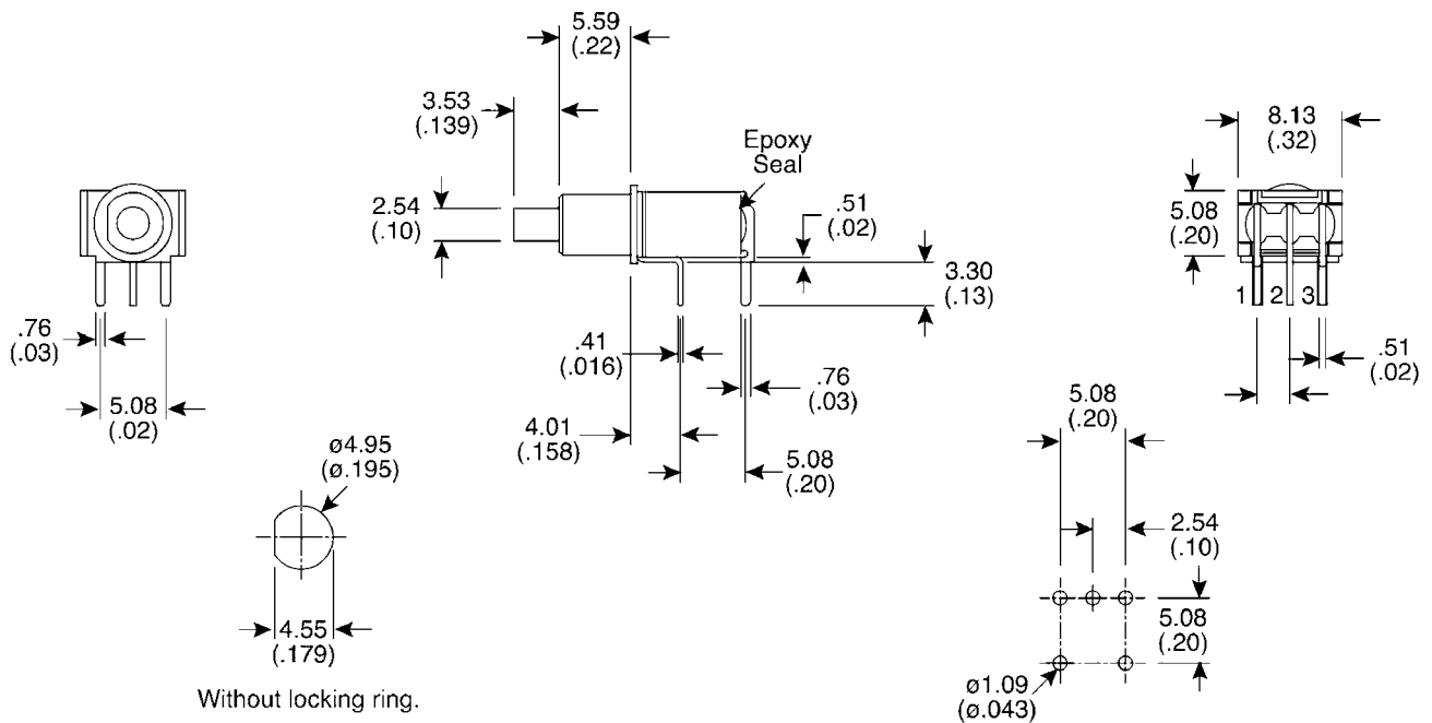
PANEL MOUNTING
